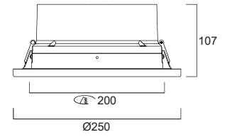
Solstice 200 Round IP65
